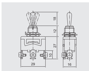
Type 1322 AC250V 15A ON-OFF-ON
