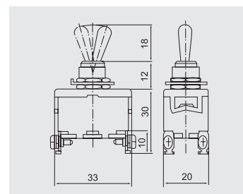
Type 1121 AC250V 15A ON-OFF
