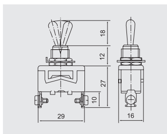
Type 1021 AC 250V 15A ON-OFF
