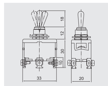
Type 1321 AC250V 15A ON-OFF-ON
